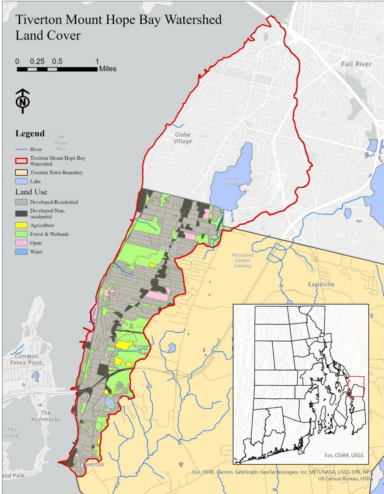
Figure 3. Land Cover
